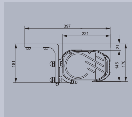
Ceiling installation, bracket backwards
