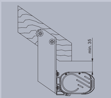
Rafter installation
